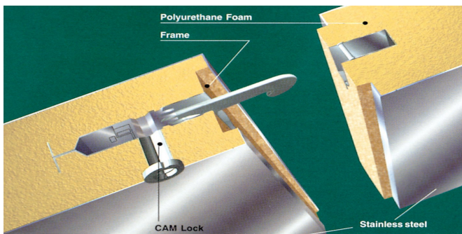
Easy Assembling at Site by Cam Lock System
